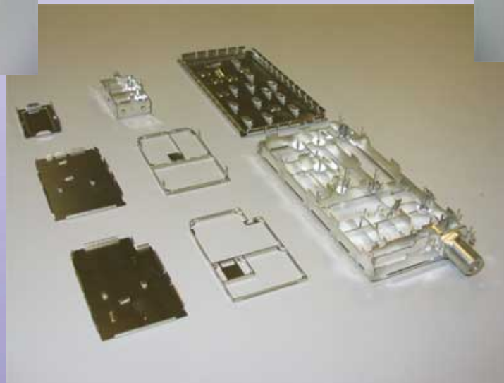
SHIELDS FOR TELECOMMUNICATION MODULES
