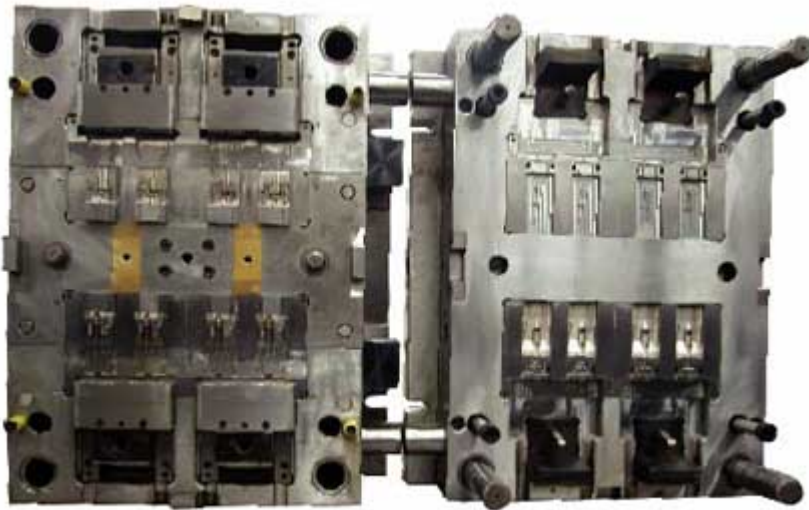
2-Component Electrical Connector Tooling
